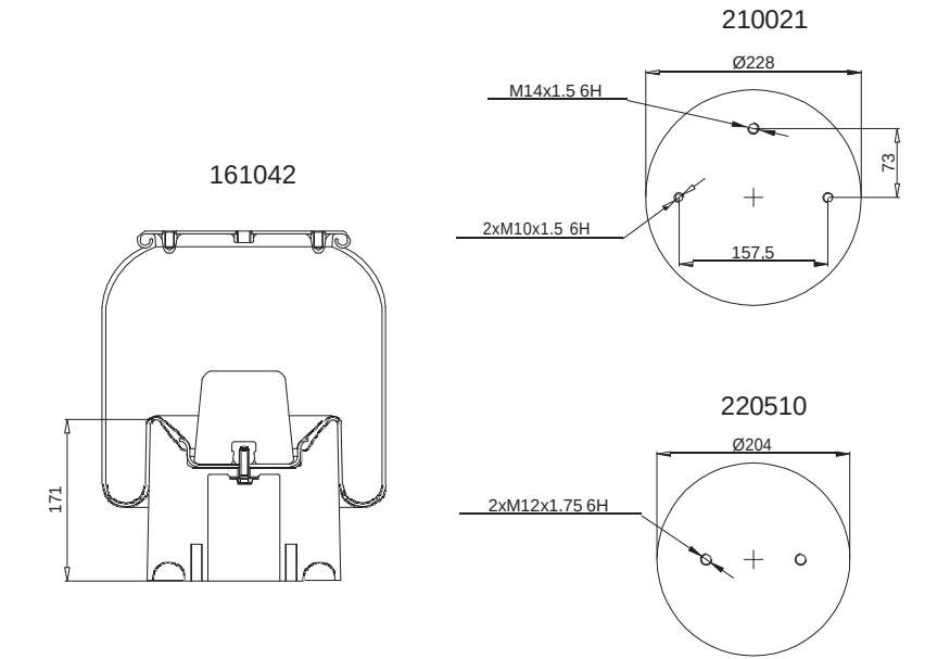
(Composite Piston)
